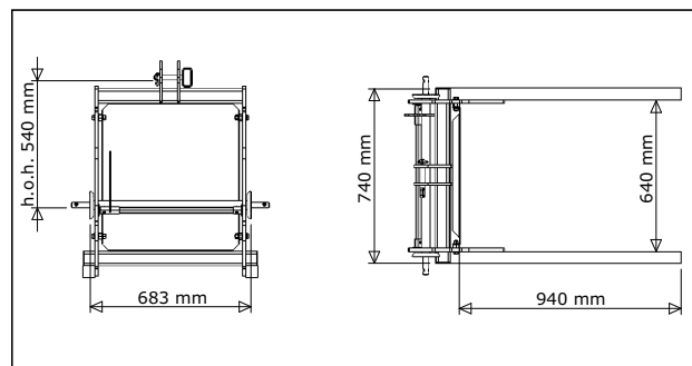
↑ Palletdrager C-1
